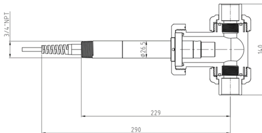
Figure 5 - ST-773 installed in the ST-001 + Collar Tee Assembly Kit (P/N 53726)
