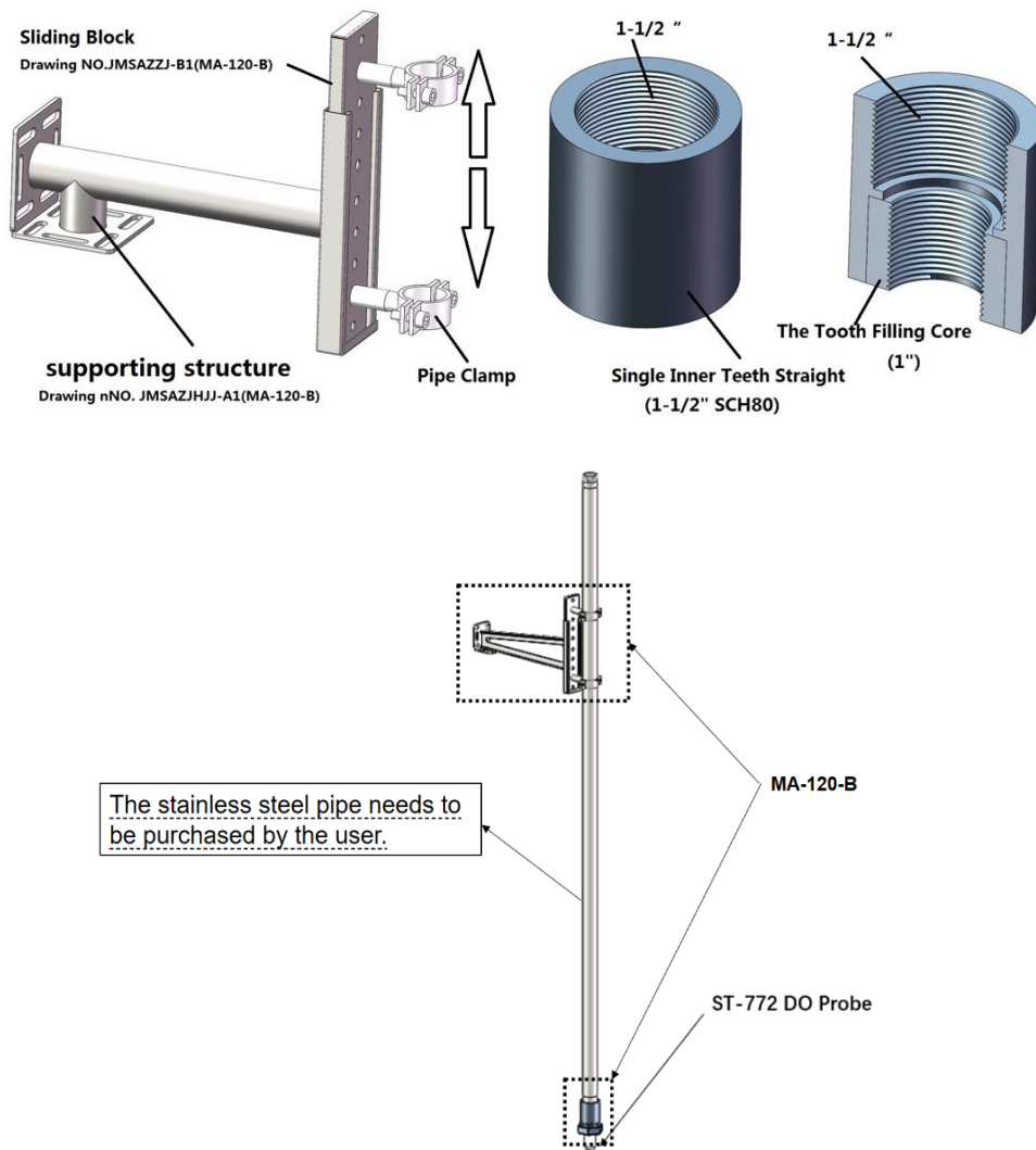
Figure 3 ST-773 in a submersed fixed installation
